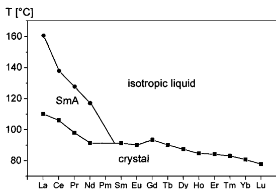
Figure 7. Phase diagram for the lanthanide(III) dodecanoates
