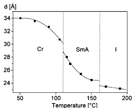
Figure 6. Evolution of the d -spacing of La III dodecanoate as a function of temperature
