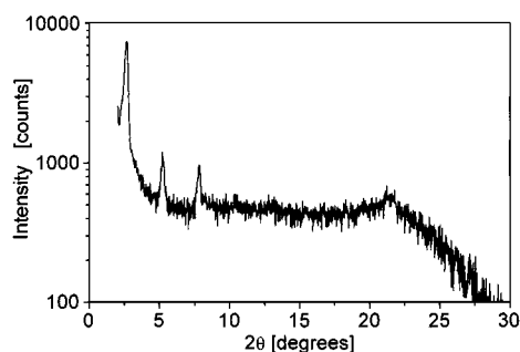
Figure 2. X-ray powder diffractogram of La III dodecanoate at 50 °C
