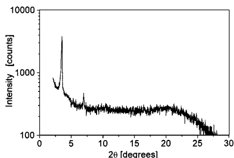
Figure 3. X-ray diffractogram of La III dodecanoate in the mesophase at 135 °C
