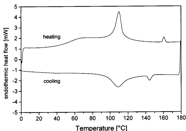
Figure 1. DSC thermogram of La III dodecanoate (first heating-cooling cycle); endothermic peaks are shown pointing upwards
