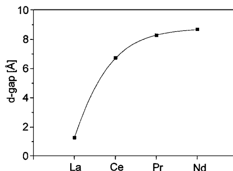
Figure 4. Variation of the change in the d -spacing at the melting point for the mesomorphic lanthanide(III) dodecanoates
