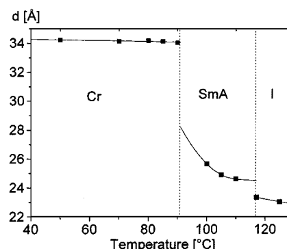
Figure 5. Evolution of the d -spacing of Nd III dodecanoate as a function of temperature
